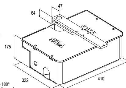
DIMENSIONS (mm)
