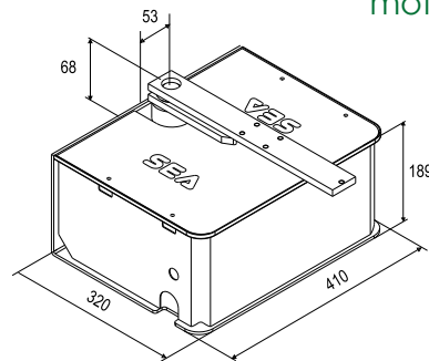
DIMENSIONS (mm)
